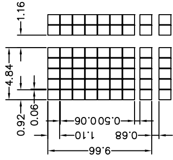
DOT DETAIL SCALE 4:1
